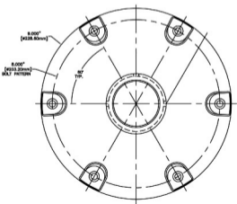
BASE MOUNTING PATTERN
